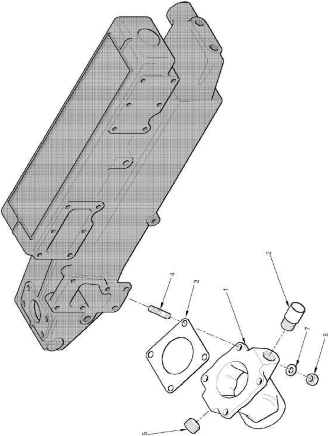
EXHAUST OUTLET, WET X 3" GROUP 6498
