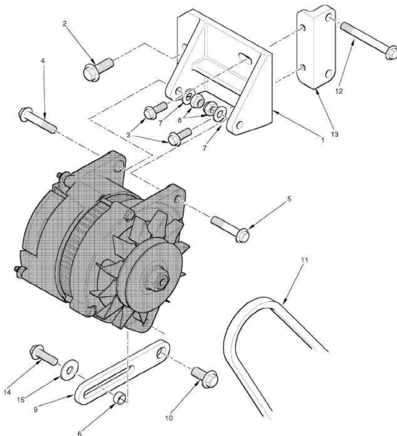
Belt, mounting brackets and hardware, A127/AS128 alternator GROUP 6485
