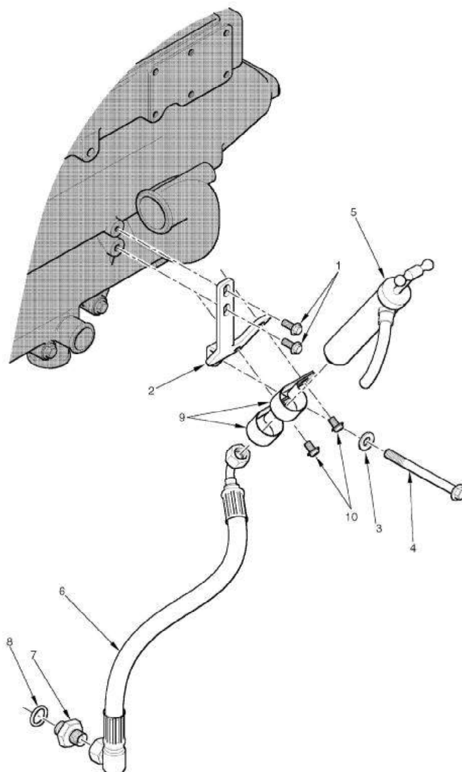
Sump pump, hose and mounting bracket GROUP 6869
